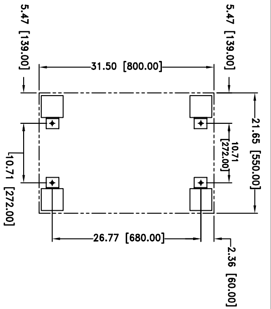
FOOT AND TIE DOWN BRACKET HOLE PATTERN
